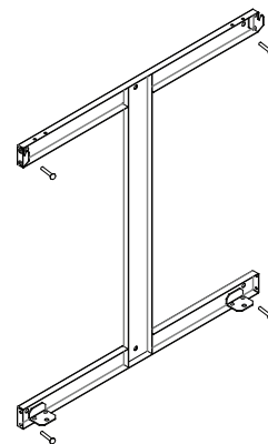
#5 Hanging Bracket
